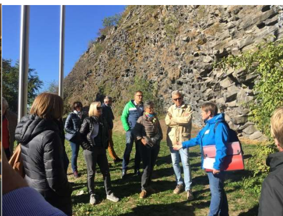
Basaltwand Parkstein
